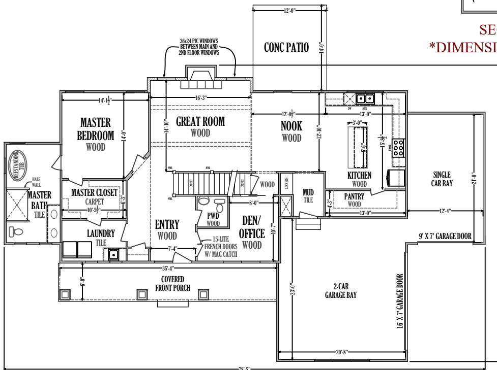
MAIN FLOOR PLAN - 1635 sq. ft.
