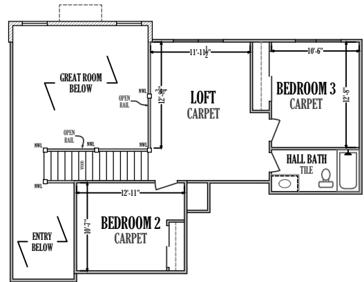
SECOND FLOOR PLAN - 657 sq. ft.
