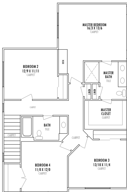
SECOND FLOOR PLAN - 1208 sq. ft.
