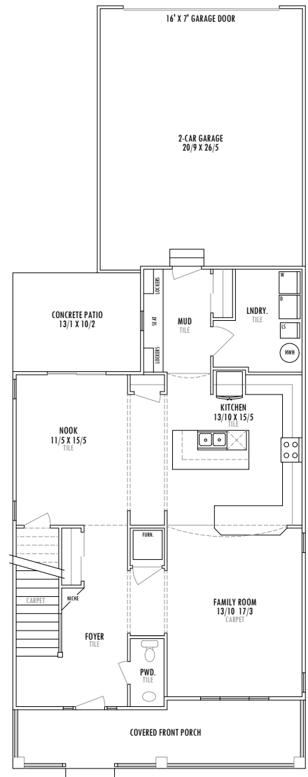
MAIN FLOOR PLAN - 1208 sq. ft.
