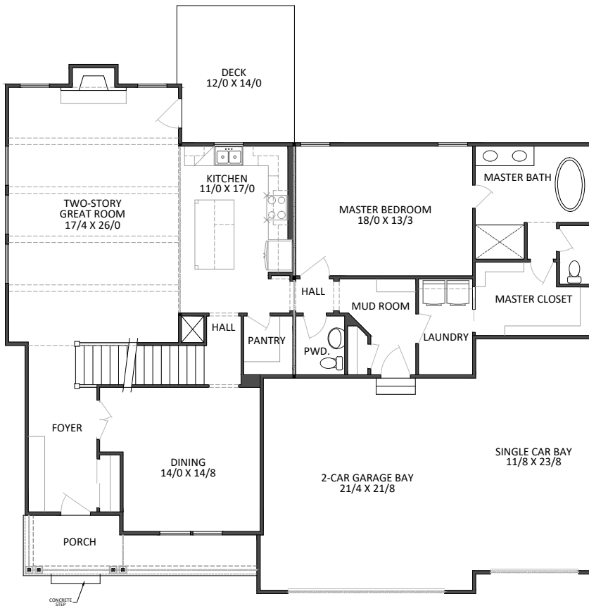
MAIN FLOOR PLAN - 1863 sq. ft.
