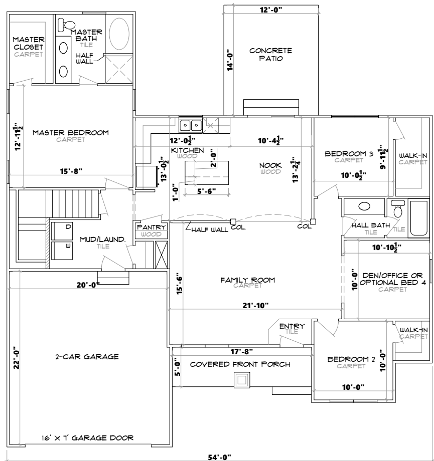
MAIN FLOOR PLAN - 1696 sq. ft.
