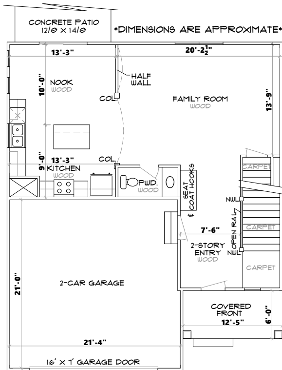
MAIN FLOOR PLAN - 825 sq. ft.
