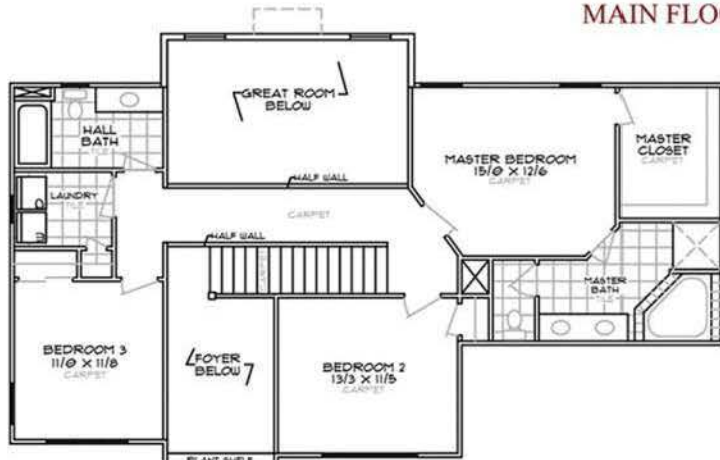
SECOND FLOOR PLAN - 1049 sq. ft.
