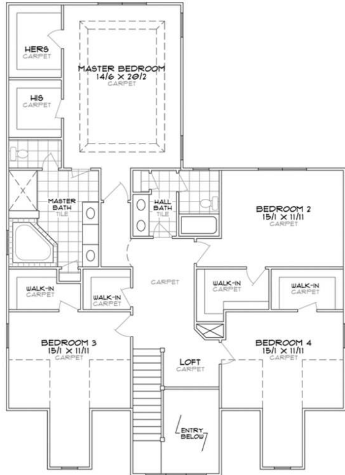
The Walter 3400 Second Floor Plan
