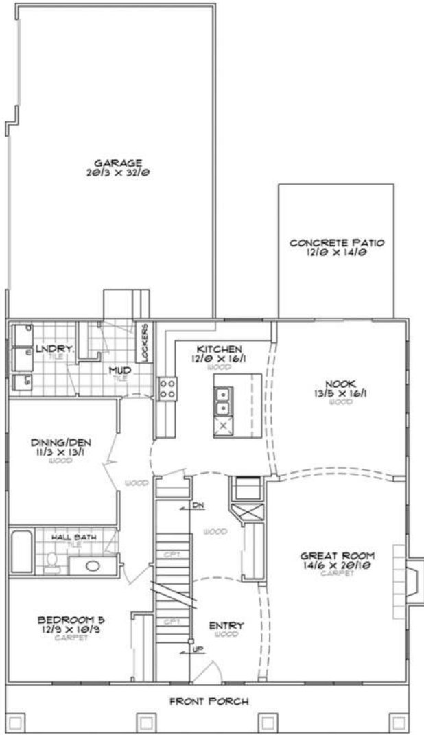
The Walter 3400 Main Floor Plan
