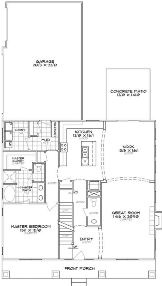
The Walter 2900 Main Floor Plan
