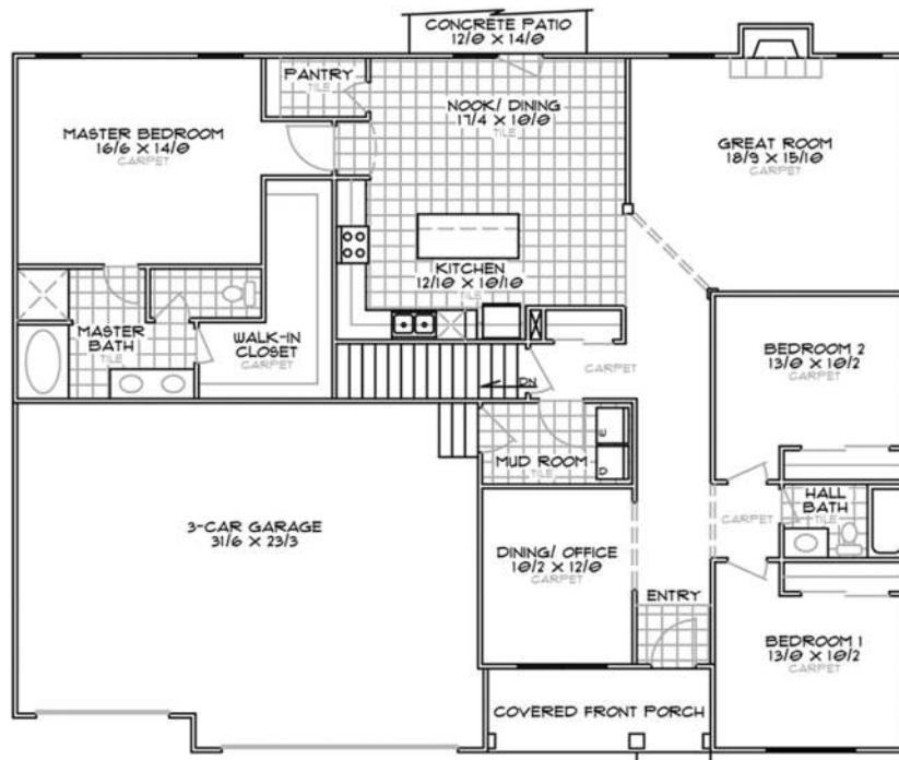
MAIN FLOOR PLAN - 2041 sq. ft.
