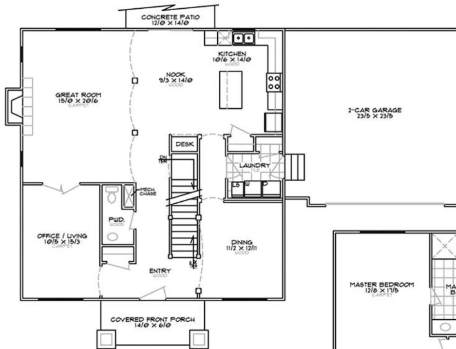
MAIN FLOOR PLAN - 1307 sq. ft.
