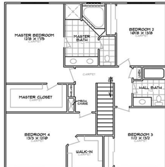
SECOND FLOOR PLAN - 1307 sq. ft.
