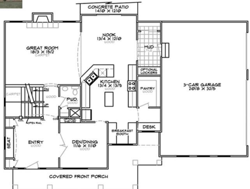
MAIN FLOOR PLAN - 1308 sq. ft.
