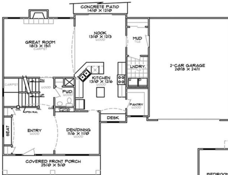
MAIN FLOOR PLAN - 1252 sq. ft.
