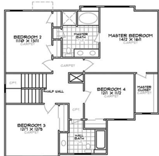
SECOND FLOOR PLAN - 1261 sq. ft.
