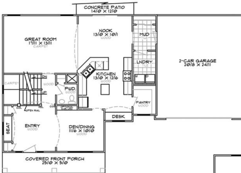
MAIN FLOOR PLAN - 1158 sq. ft.
