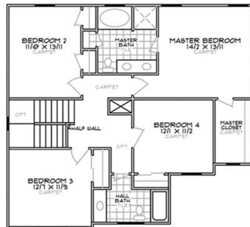
SECOND FLOOR PLAN - 1166 sq. ft.
