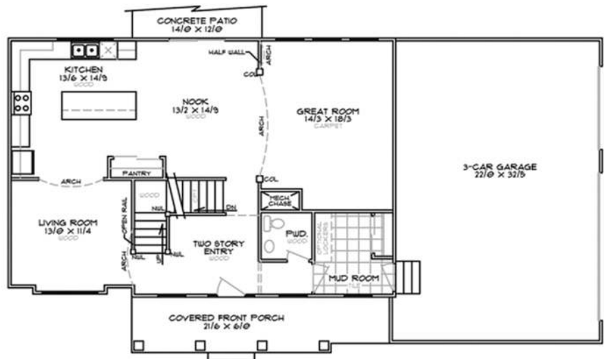
MAIN FLOOR PLAN - 1158 sq. ft.
