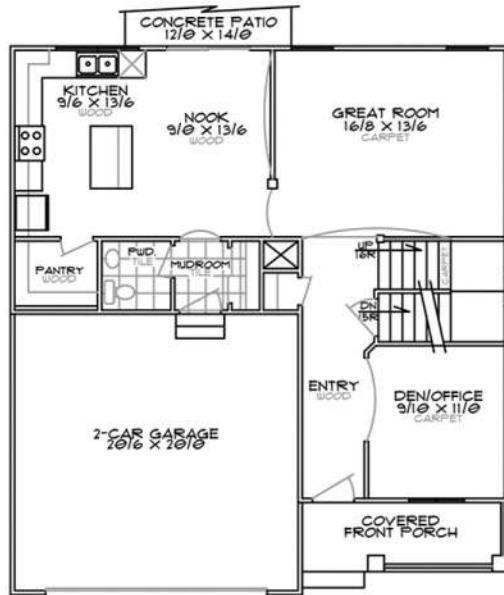
MAIN FLOOR PLAN - 904 sq. ft.
