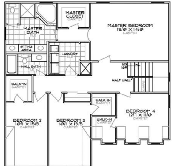
SECOND FLOOR PLAN - 1492 sq. ft.
