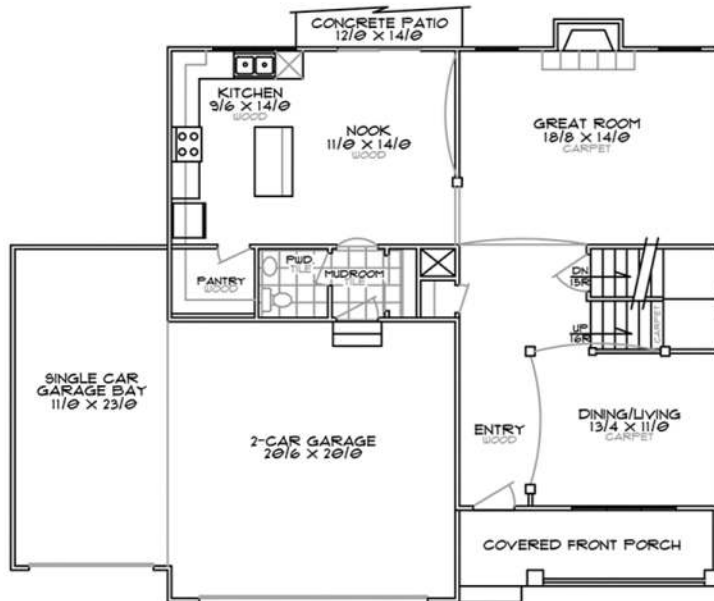
MAIN FLOOR PLAN - 1056 sq. ft.
