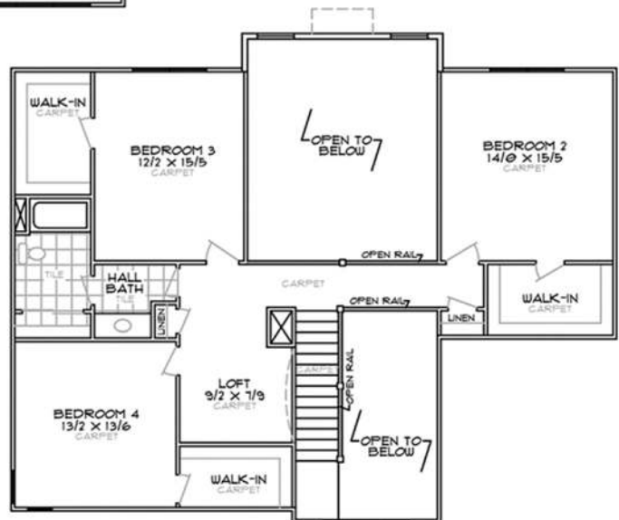
SECOND FLOOR PLAN - 1213 sq. ft.
