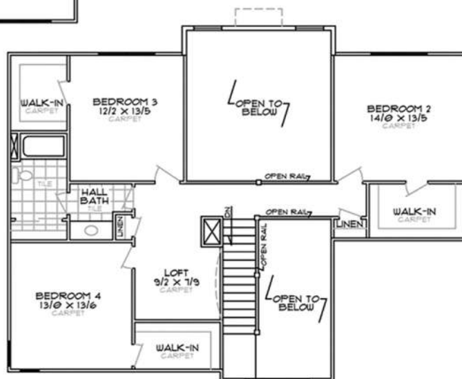
SECOND FLOOR PLAN - 1139 sq. ft.
